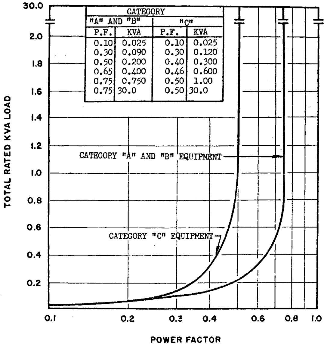
FIGURE 8. Lagging power factor limits for utilization equipment
